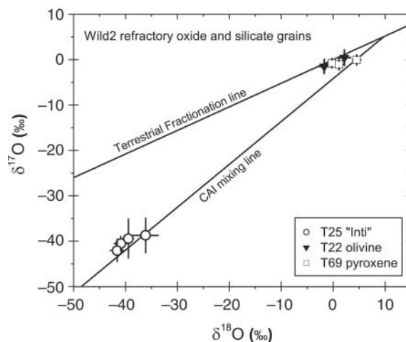
Fig. 4. Oxygen isotopic compositions of individual cometary grains. The terrestrial mass-dependent fractionation line (TF) and the CAI-mixing line are shown for reference. Error bars are 2\sigma .
