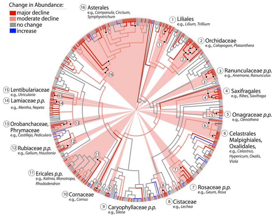
Fig. 1. Composite phylogeny of 429 flowering plant species from the Concord flora depicting changes in abundance from 1900 to 2007. Change in abundance ranged on an integer scale from 5 to 0, and was calculated as the difference in abundance for each taxon in 1900 and 2007 based on 7 abundance categories (0 to 6; see Materials and Methods ). Branch color indicates parsimony character state reconstruction of change in abundance. For simplicity, we have indicated this reconstruction by using 4 colors: red (major decline, 5 to 3), pink (moderate decline, 2), gray (little to no change, 1 to 0), and blue (increase, 0 to 1). For the complete character reconstruction and taxon labels see Fig. S1. Average decline in abundance was calculated for all internal nodes as the mean change in abundance of descendant nodes weighted with branch length information ascertained from divergence time estimates. An average decline of 2.5 or greater corresponds to a decline in abundance of 50% or greater, based on our most conservative scoring using 6 abundance categories (0 to 5; see Materials in Methods ). Clades exhibiting these major declines are indicated with black dots. Each of the most inclusive clades exhibiting these declines are indicated in pink and referenced numerically to their clade name. Subclades in major decline that are nested within more widely recognized clades are labeled with the more familiar name followed by pro parte ( p.p. ). These clades include some of the most charismatic wildflower species in New England, such as anemones and buttercups ( Ranunculaceae p.p. ), asters, campanulas, goldenrods, pussytoes, and thistles ( Asterales ), bedstraws and bluetts ( Rubiaceae p.p. ), bladderworts ( Lentibulariaceae ), dogwoods ( Cornaceae ), lilies ( Liliales ), louseworts and Indian paintbrushes ( Orobanchaceae ), mints ( Lamiaceae p.p. ), orchids ( Orchidaceae ), primroses ( Onograceae p.p. ), roses ( Rosaceae p.p. ), saxifrages ( Saxifragales ), Indian pipes ( Ericales p.p. ), and St. John's worts and violets ( Malpighiales ).
